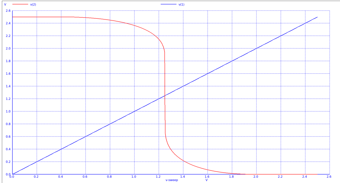
Figure 17: Voltage transfer characteristic of symmetrical CMOS inverter
